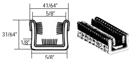
Universal Single Channel
