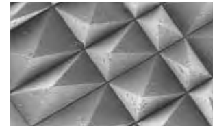
The precisely structured surface of Trizact™ film is clearly visible under 50X magnification
