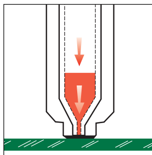
Hydraulic pressure forces resin into the cavity
