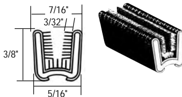
Universal Single Channel
