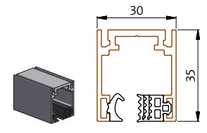
Top-Frame
